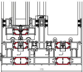
Sill Detail
